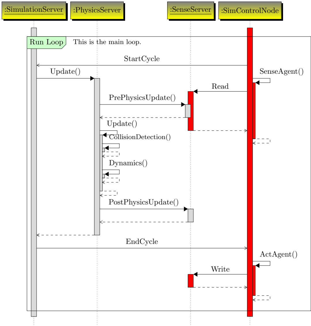
Figure 2: Example of a sequence with parallel activities. The used style-file is part of pgf-umlsd-0.2.tar.gz – get it at http://code.google.com/p/pgf-umlsd/
