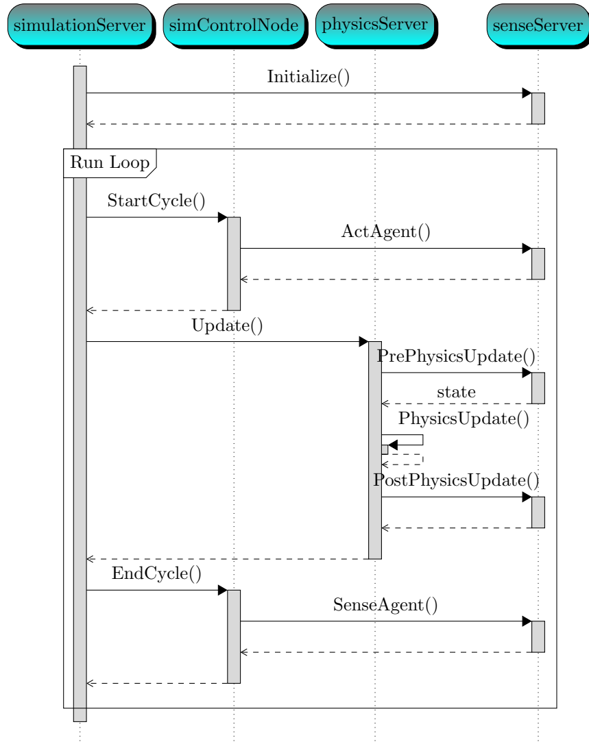
Figure 1: UML sequence diagram demo. The used style-file is part of pgf-umlscd-0.2.tar.gz Get it at http://code.google.com/p/pgf-umlscd/
